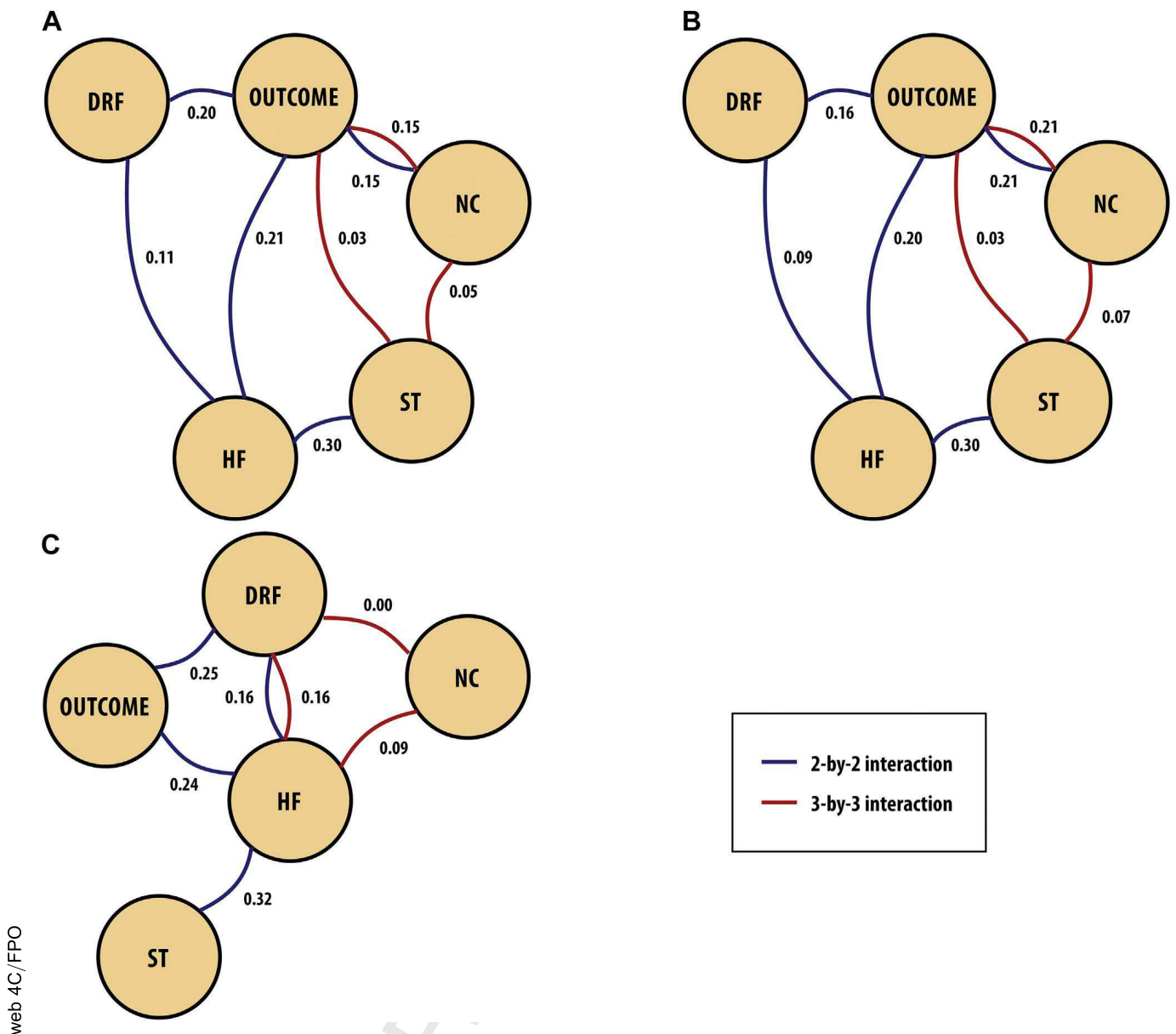
Figure 2. Graphical log-linear model and graphical random forests (GRaFo) representation. (A) 1978-2015, (B) 1978-1999, and (C) 2000-2015. 045 The weights on the edges correspond to Cramer's V coefficients (V). Outcome = death. This representation assesses the degree of dependence between the variables (complications and death). In the analysis of (A) the whole cohort, for the 2-by-2 interaction ( blue lines ), heart failure (HF) was associated with dialysis-dependent renal failure (DRF) ( V = 0.11 ) and with surgical treatment (ST) ( V = 0.30 ). Neurologic complications (NC), HF, and DRF were associated with mortality ( V = 0.21, 0.20, 0.15 , respectively). For the 3-by-3 interaction ( red lines ) of mortality, ST, and NC, a greater dependence between mortality and NC ( V = 0.15 ) was observed. The dependence relationships found in (A) and (B) are the same. In the 2000-2015 group (C) , there is a dependence relationship between surgical treatment and mortality, conditioned to the presence of HF and of the other variables.
